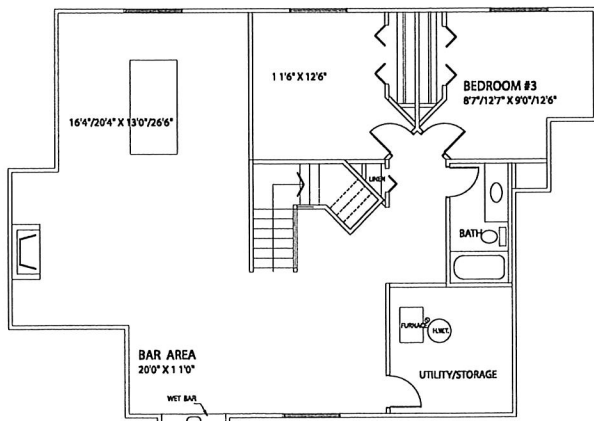
BASEMENT PLAN - 1281 SQ. FT.
